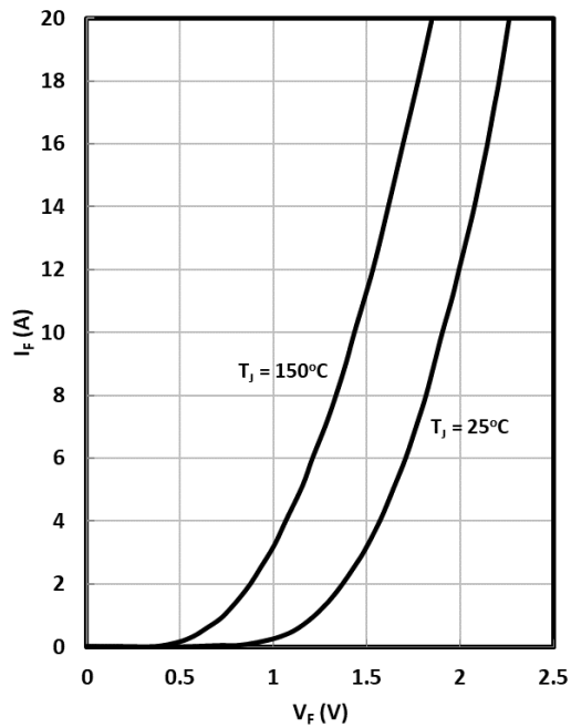
Fig. 13 Diode (Brake-Chopper) Output Characteristics
