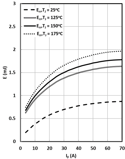
Fig. 9 Diode (Inverter) switching loss vs. I_F ( V_{CC} = 600V , R_G = 5\Omega )
