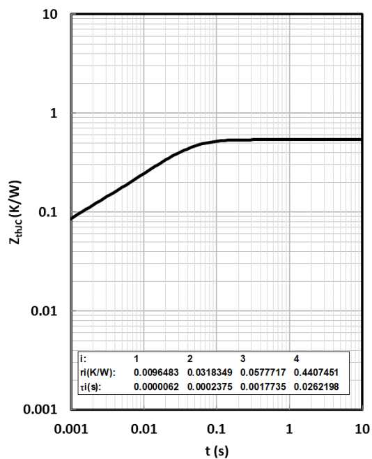
Fig. 7 IGBT (Inverter) Transient Thermal Impedance
