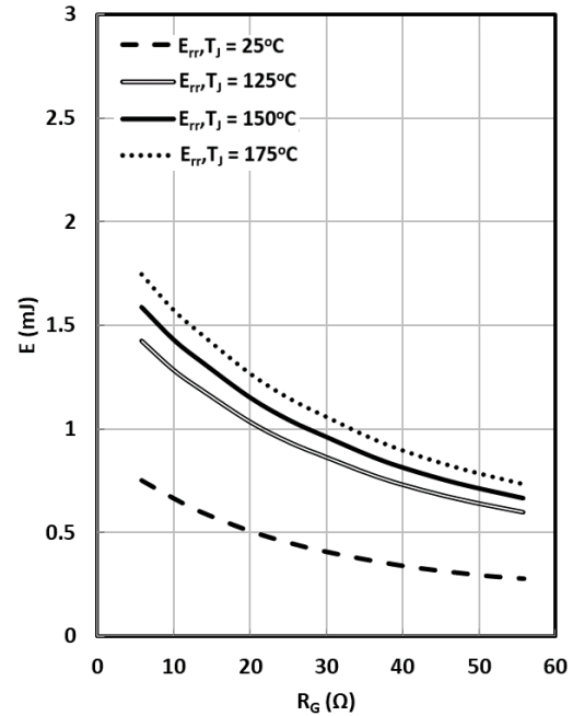
Fig. 10 Diode (Inverter) switching loss vs. R_G ( V_{CC} = 600V , I_F = 35A )
