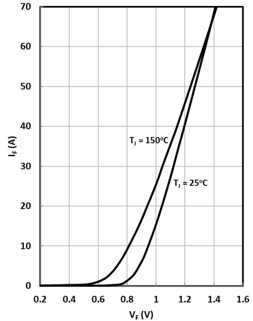
Fig. 14 Diode (Rectifier) Forward Characteristics
