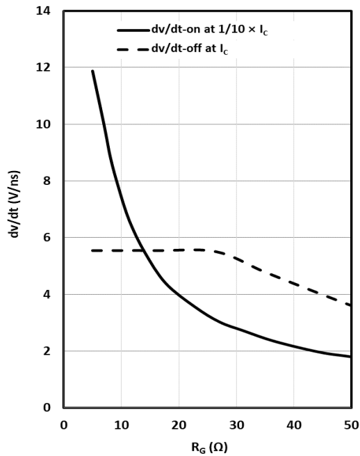
Fig. 5 IGBT (Inverter) dv/dt ( V_{CC} = 600V , V_{GE} = \pm 15V , I_C = 35A )
